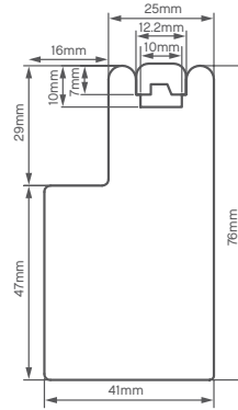
Builtout L Frame with Cap (41 x 76mm)
