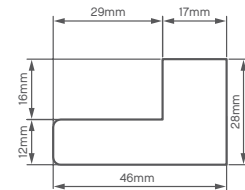
L Frame Sill
