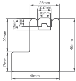
L Frame with Cap
