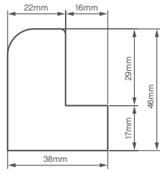
Bullnose L Frame
