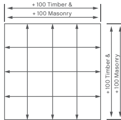
Face Fit - no architrave
