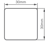
Mounting Strip (With or without cap)
