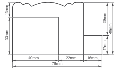
Gallery Z Frame
