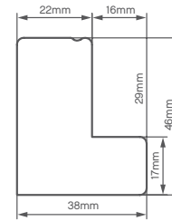
Beaded L Frame
