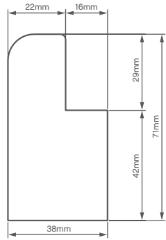
Builtout Bullnosed L Frame (38 x 78)
