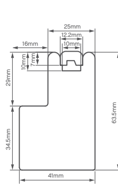
Builtout L Frame with Cap (41 x 63.5mm)
