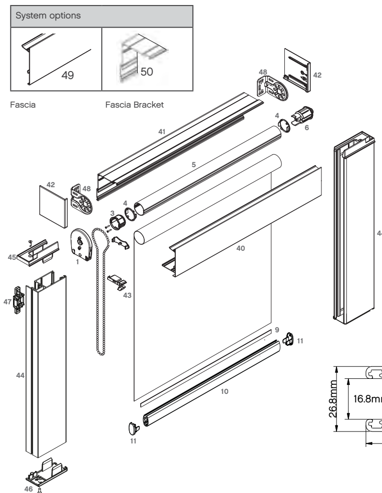
Exploded view diagram of headbox with side guide
